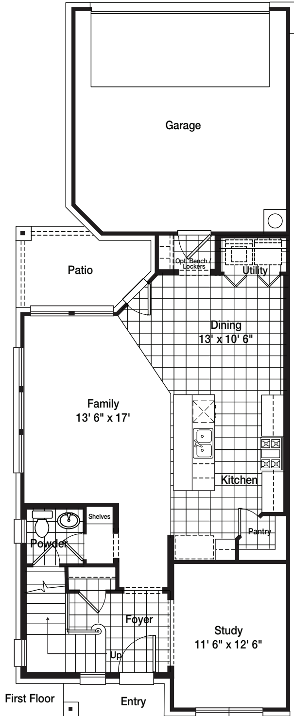
Floor Plan
