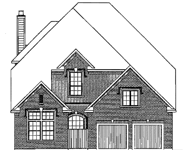
ELEVATION C
