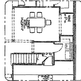
FIRST FLOOR PLAN OPTIONS
