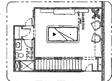
SECOND FLOOR PLAN OPTIONS
